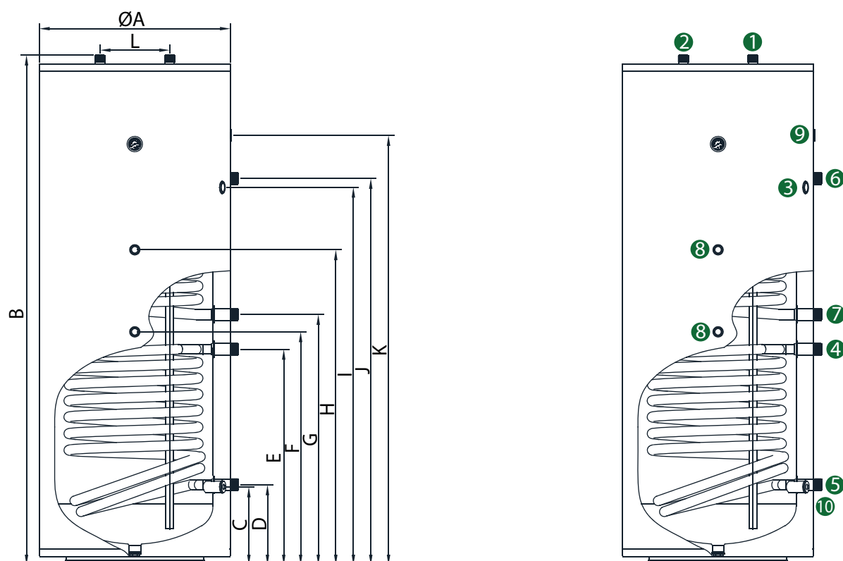
Figure 4 - Double Coil - Upper connections
