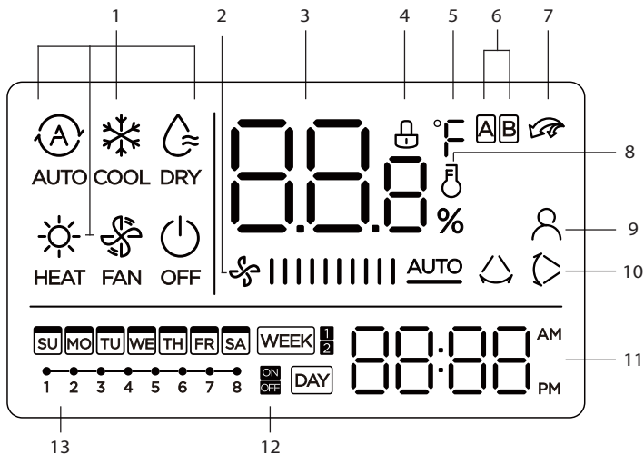
Fig. 3 — Wired Controller Display
